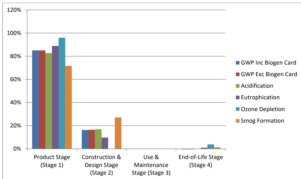
Figure 2. Impact Category Result Breakdown by ISO 21930 Stage for Average TUFF SURFACE Formulation.
