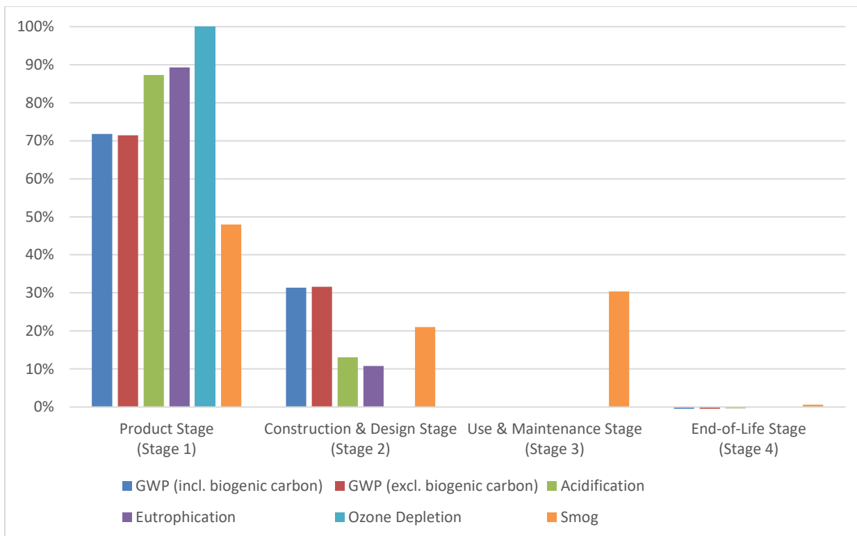
Figure 2. Impact Category Result Breakdown for the CONFLEX™ Block Filler Formulation.
